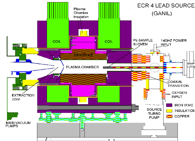
CERN Lead source
