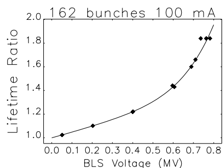
Figure 9: Lifetime as a function of BLS voltage measured at 100 mA with 162 bunches. Lifetime at zero voltage is 1.5 hours.
